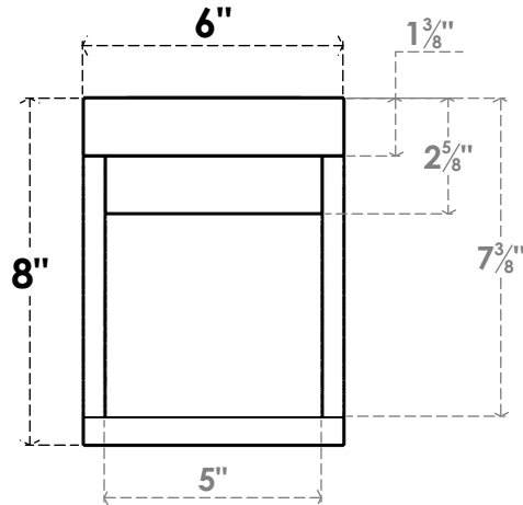
FRONT PROFILE
